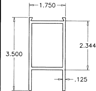
② BOTTOM RAIL (NARROW STILE)
