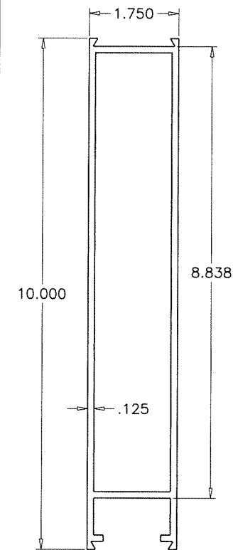
②C 10" BOTTOM RAIL (OPTIONAL FOR NARROW, MEDIUM AND WIDE STILE DOORS)
