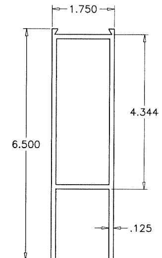
②B BOTTOM RAIL (MEDIUM & WIDE STILE)
