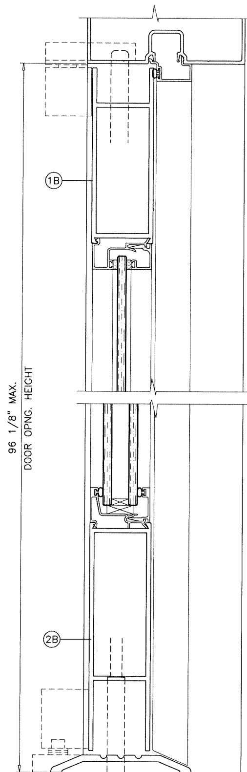
WIDE STILE DOOR
